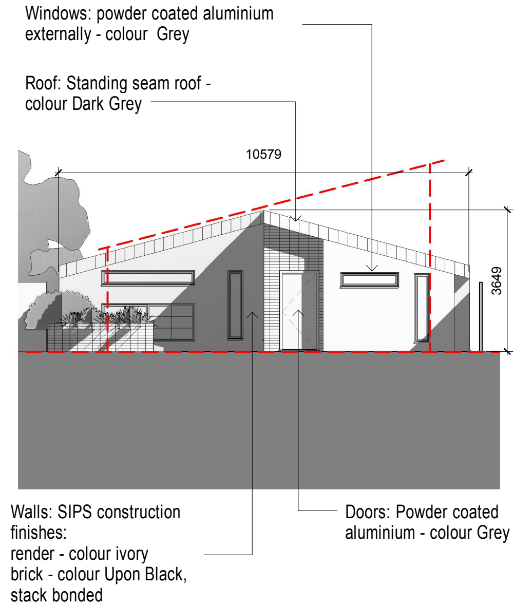
South West Facing Elevation 1 : 100
